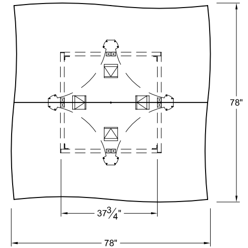
PLAN VIEW-QUAD BASE
