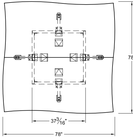
PLAN VIEW-CASTER BASE
