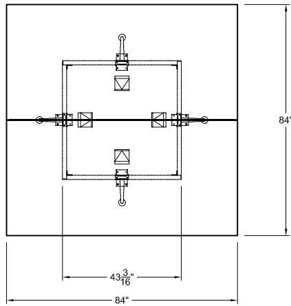
PLAN VIEW-TAPER BASE
