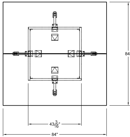
PLAN VIEW-CASTER BASE
