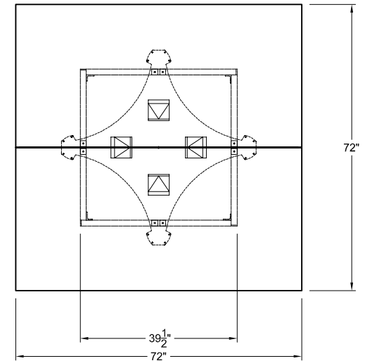
PLAN VIEW-QUAD BASE
