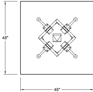
PLAN VIEW-TAPER BASE
