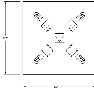
PLAN VIEW-CASTER BASE
