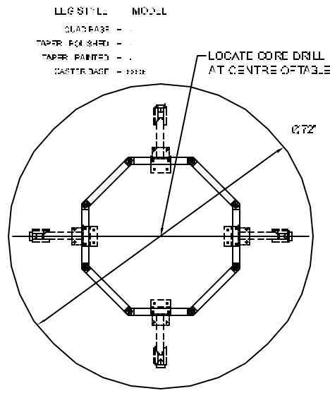
PLAN VIEW-CASTER BASE
