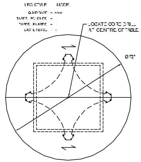
PLAN VIEW-QUAD BASE
