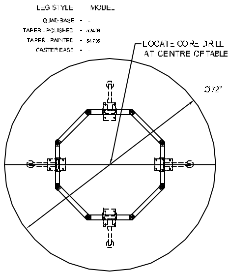
PLAN VIEW-TAPER BASE
