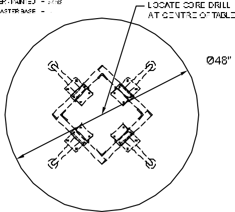
PLAN VIEW-TAPER BASE
