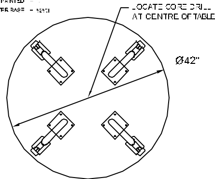
PLAN VIEW-CASTER BASE
