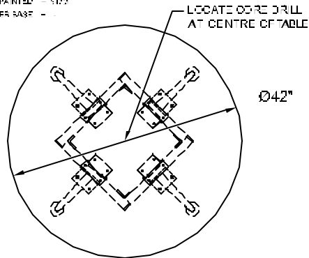
PLAN VIEW-TAPER BASE
