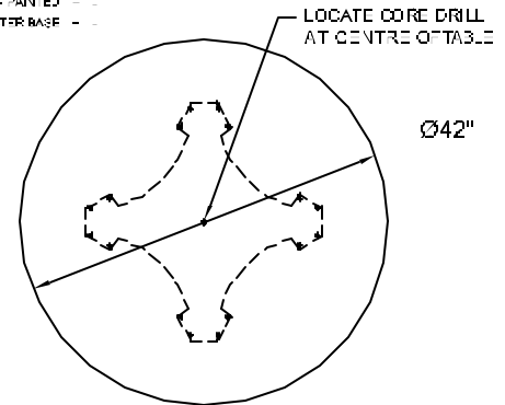
PLAN VIEW-QUAD BASE
